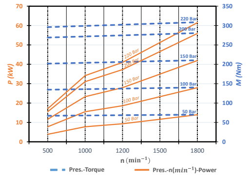
Flow-rpm Graphic
