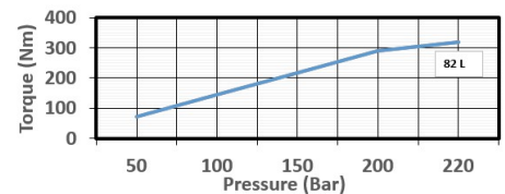
Torque-Pressure Graphic
