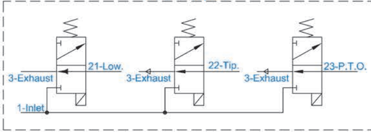
Pnömatik Sembol Pneumatic Symbol
