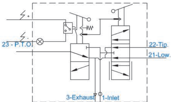
Pnömatik Sembol Pneumatic Symbol
