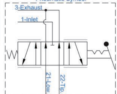
Pnömatik Sembol Pneumatic Symbol
